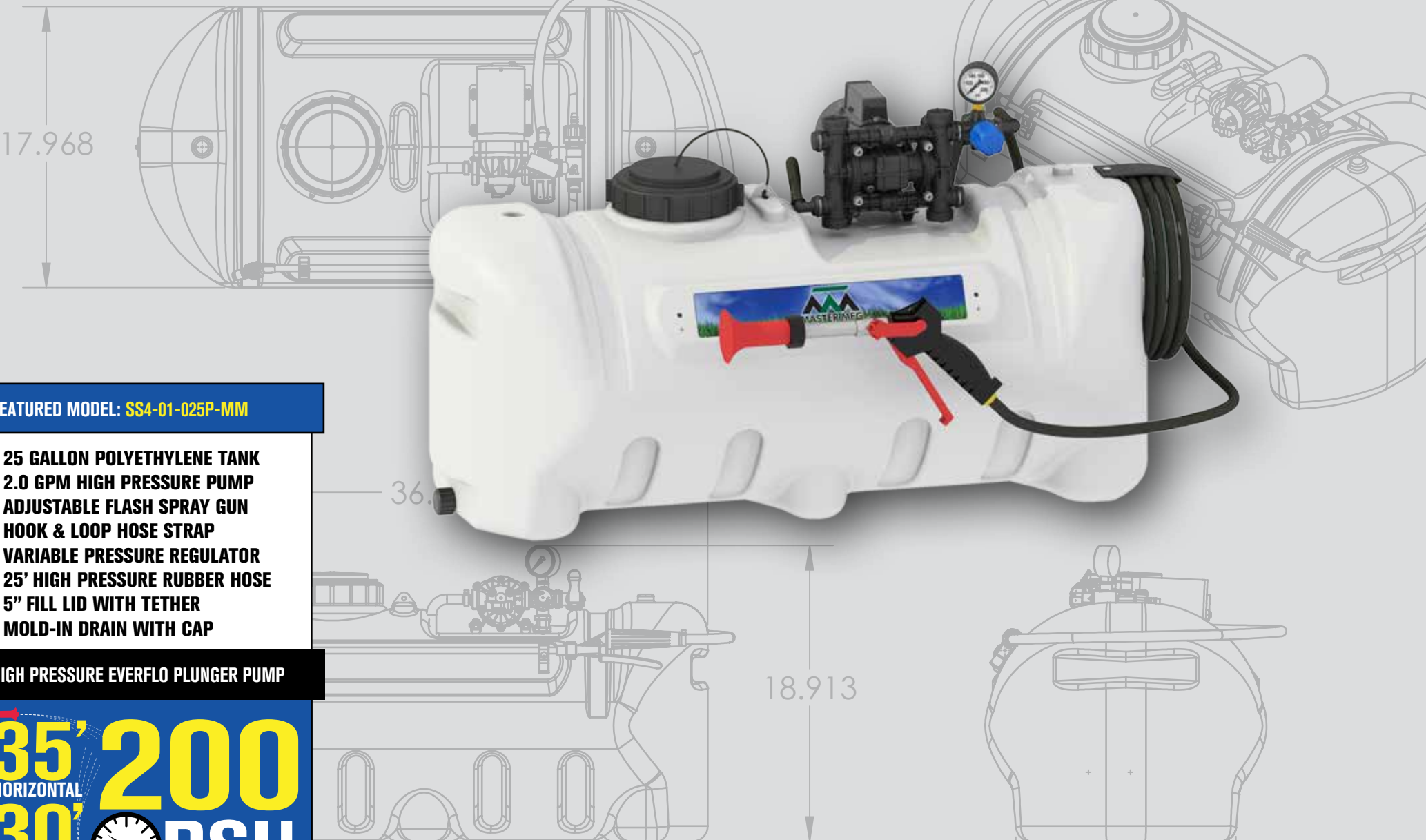
25 GALLON TREE SPRAYER
